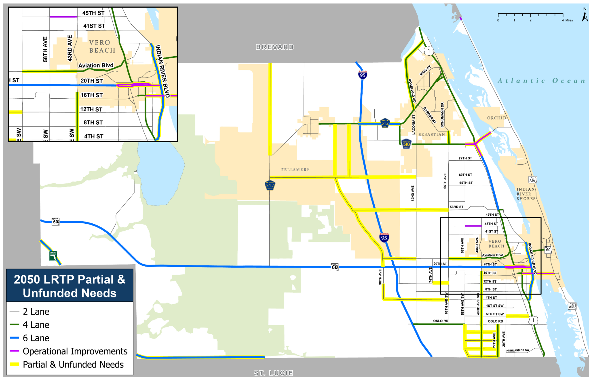
Figure 4-4. Partially and Unfunded 2050 Unfunded Roadway Needs
